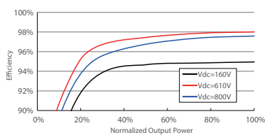
SG 3KTL-EC
