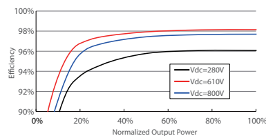
SG 5KTL-EC
